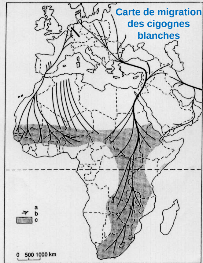
Fig. 17. Schematic representation of the two main migration routes of the White stork ( Ciconia ciconia ) across the Iberian peninsula in the west, and along the eastern edge of the Mediterranean in the east, with secondary migration routes. Dotted area: winter quarters (from Nowak and Berthold 1987).
